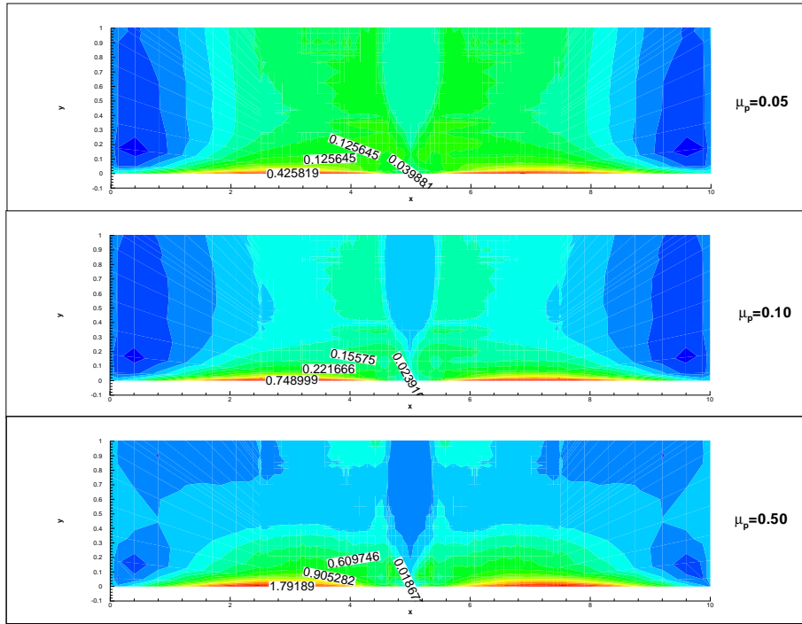
Figure 7.37: The stress contours of component T_{xx} for different polymeric viscosities. The remaining parameters are We = \mu_s = 0.1 , h = 1.1 .
