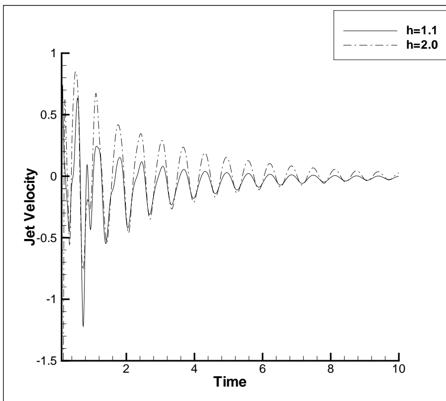
Figure 7.29: Variation of the jet velocity with time, at different distances h from the wall, in a UCM fluid with \mu_p = 0.1 , We = 0.03 .
