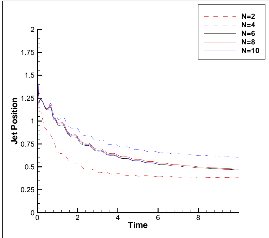
Figure 7.20: Dependence of the position of the jet on mesh refinement for \mu_s = 0.1 .
