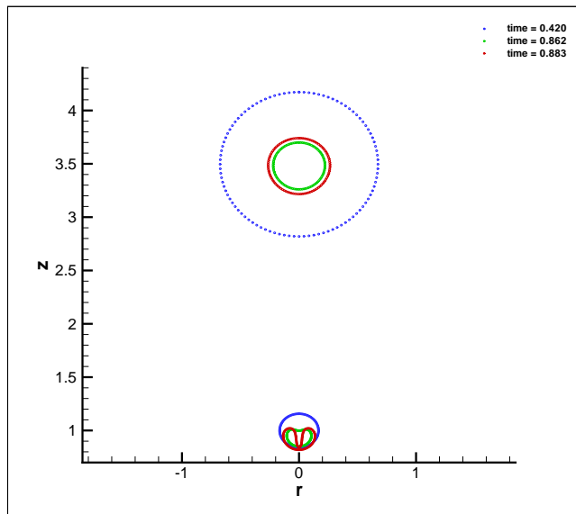
Figure 4.31: Bubble shapes for De = 1 , Re = 2 , h_1 = 1.0 , h_2 = 3.5 . Different colours indicate different instances in time.
