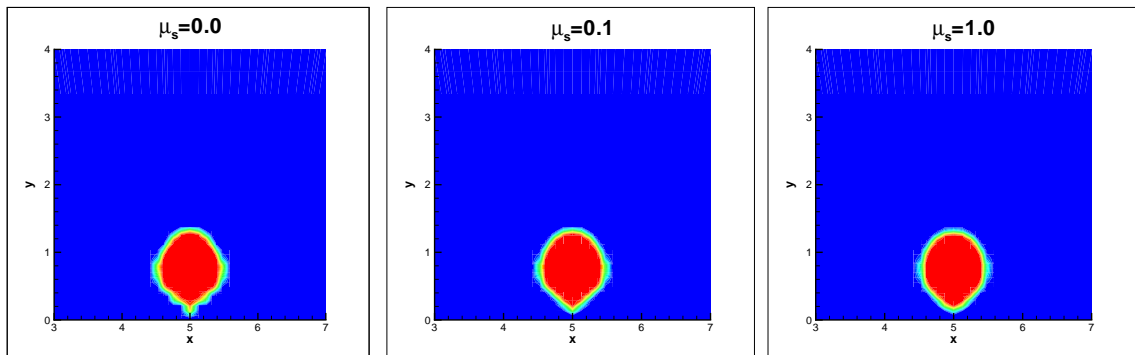
Figure 7.30: A plot of the colour function at t = 0.5 in an Oldroyd B fluid for different solvent viscosities \mu_s . The remaining parameters are \mu_p = 0.1 , We = 0.03 , h = 1.1 .
