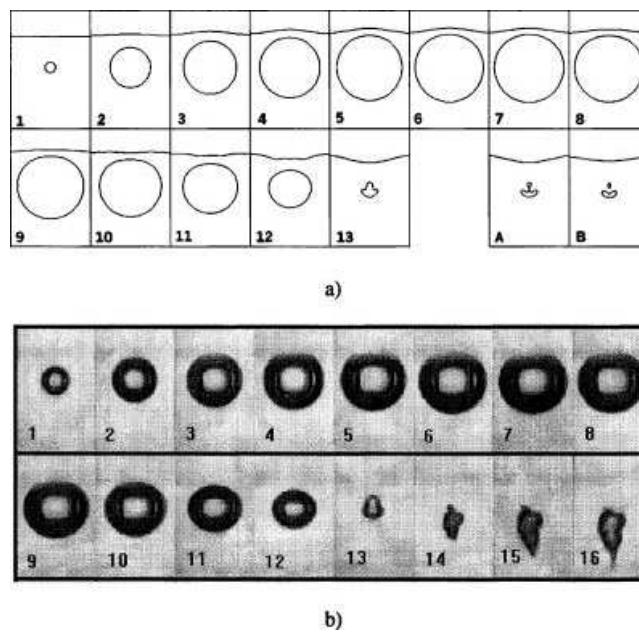
Figure 5.39: Bubble collapse near an elastic medium 2 .
