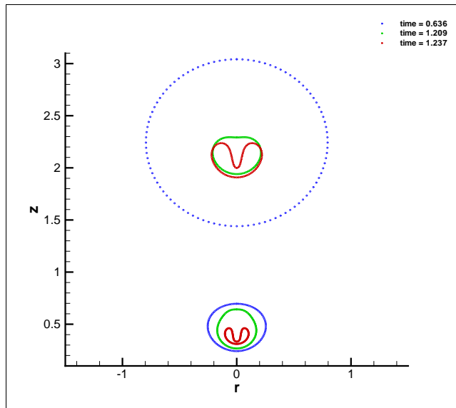
Figure 4.24: Bubble shapes for De = 2.5 , Re = 2 , h_1 = 0.5 , h_2 = 2.25 . Different colours indicate different instances in time.
