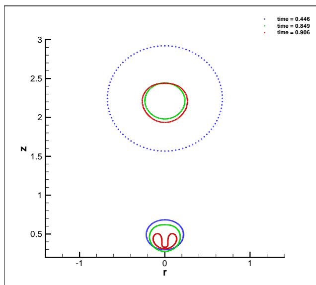
Figure 4.22: Bubble shapes for De = 1 , Re = 2 , h_1 = 0.5 , h_2 = 2.25 . Different colours indicate different instances in time.
