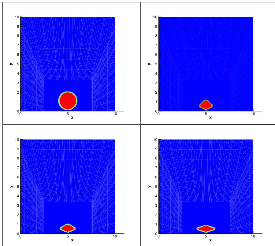
Figure 7.23: A plot of the colour function at different times, representing bubble collapse near a wall in a UCM fluid with \mu_p = 0.1 , We = 0.03 , h = 1.1 .
