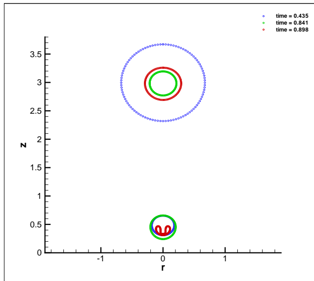
Figure 4.27: Bubble shapes for De = 1 , Re = 2 , h_1 = 0.5 , h_2 = 3.0 . Different colours indicate different instances in time.
