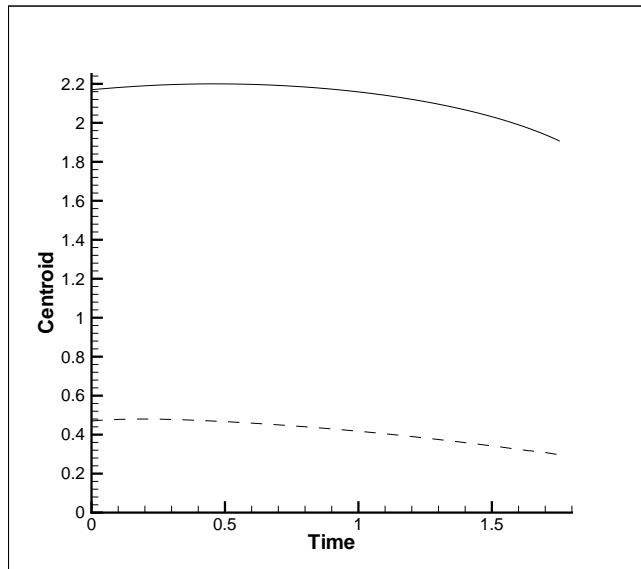
Figure 4.6: Evolution of bubble centroids. h_2 = 0.47 , h_1 = 2.17 , R_2 = 0.57 .
