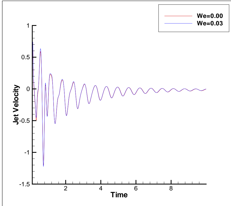
Figure 7.27: Variation of jet velocity with time (after the initial collapse) in a Newtonian and UCM fluid, \mu_p = 0.1 , h = 1.1 .
