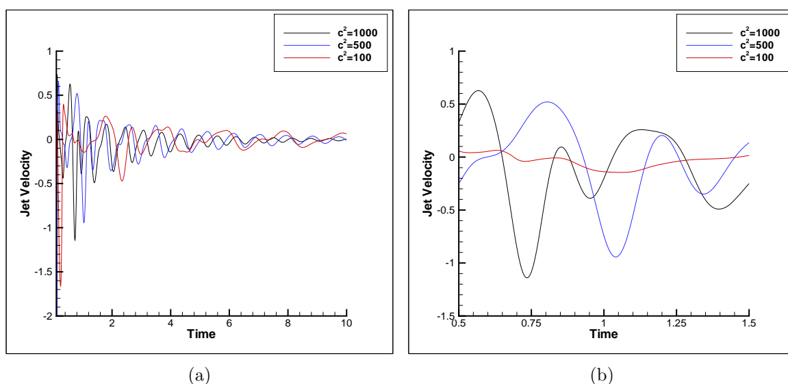
Figure 7.40: (a) Variation of jet velocity with time (after initial collapse) for different speeds of sound, with We = \mu_s = \mu_p = 0.1 , h = 1.1 . (b) Close up of the jet velocities, indicating the increase in the frequency of oscillations with increasing sound speed.
