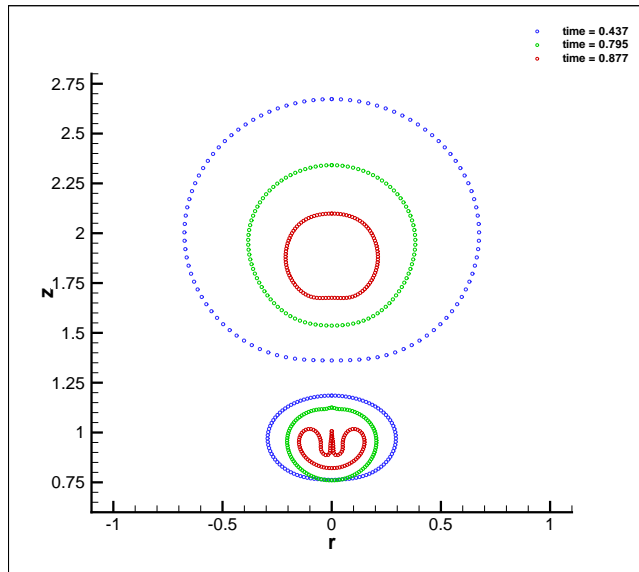
Figure 4.30: Bubble shapes for De = 1 , Re = 2 , h_1 = 1.0 , h_2 = 2.0 . Different colours indicate different instances in time.
