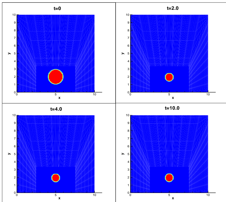
Figure 7.22: A plot of the colour function at different times, representing bubble collapse near a wall in a Newtonian fluid with \mu_s = 0.1 , h = 2.0 .
