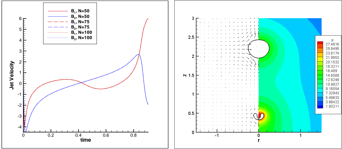
(a) North pole jet velocities for different mesh re- (b) Velocity vector and pressure contour plots at finement. t \approx 0.9 .
