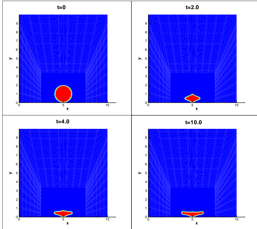
Figure 7.17: Bubble collapse near a wall in a Newtonian fluid with \mu_s = 0.1 .
