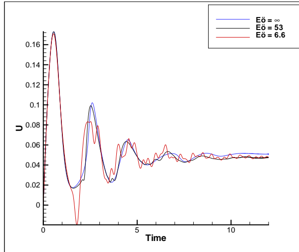
Figure 6.22: Rise velocity with time for a selection of Eötvös numbers with Re = 1.18 and De = 0.93
