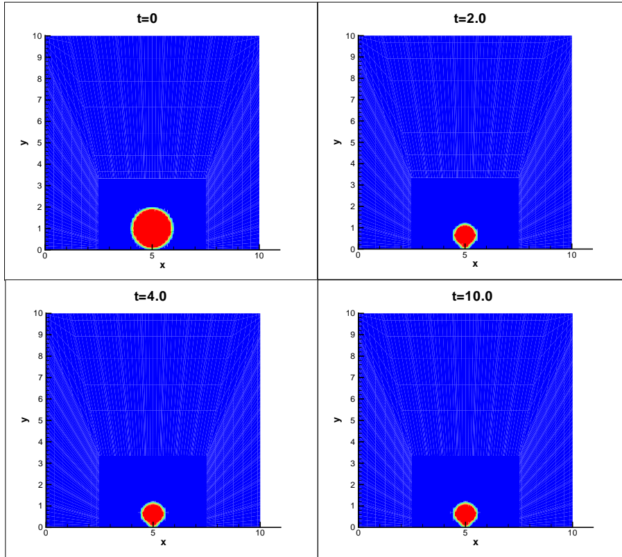
Figure 7.18: Bubble collapse near a wall in a Newtonian fluid with \mu_s = 1.0 .
