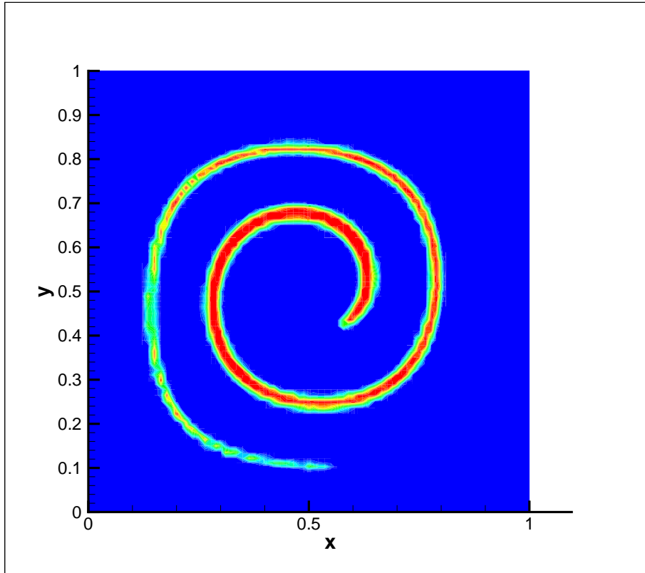
Figure 7.5: The colour function for the time reversed vortex problem at t = T_f/2 = 4.0 .
