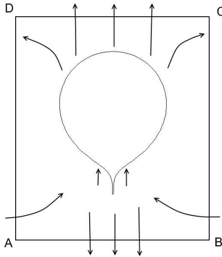
Figure 6.20: Indication of direction of velocities in rising bubble with negative wake, resulting in an additional upward thrust.
