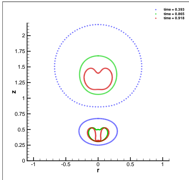
Figure 4.26: Bubble shapes for De = 1 , Re = 2 , h_1 = 0.5 , h_2 = 1.5 . Different colours indicate different instances in time.
