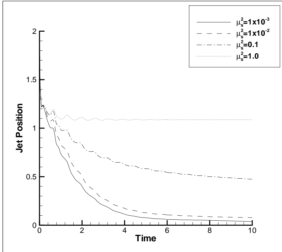
Figure 7.19: Position of jet with time for varying solvent viscosity \mu_s .
