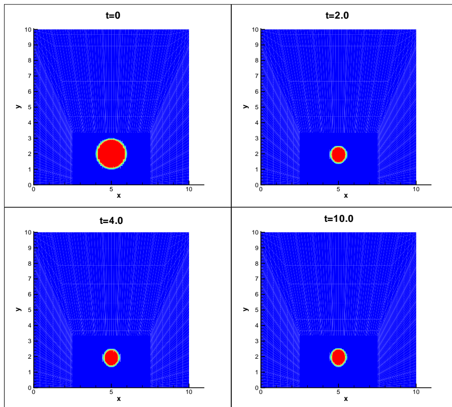
Figure 7.28: A plot of the colour function at different times, representing bubble collapse near a wall in a UCM fluid with \mu_p = 0.1 , We = 0.03 , h = 2.0 .
