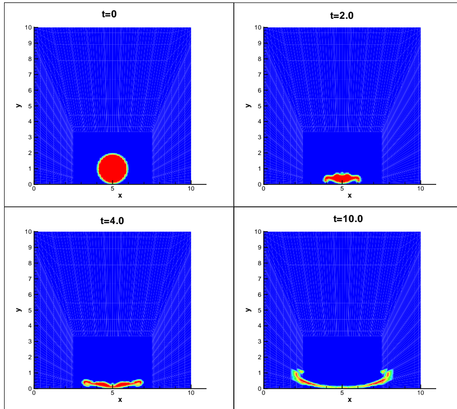
Figure 7.16: Bubble collapse near a wall in a Newtonian fluid with \mu_s = 1 \times 10^{-2} .
