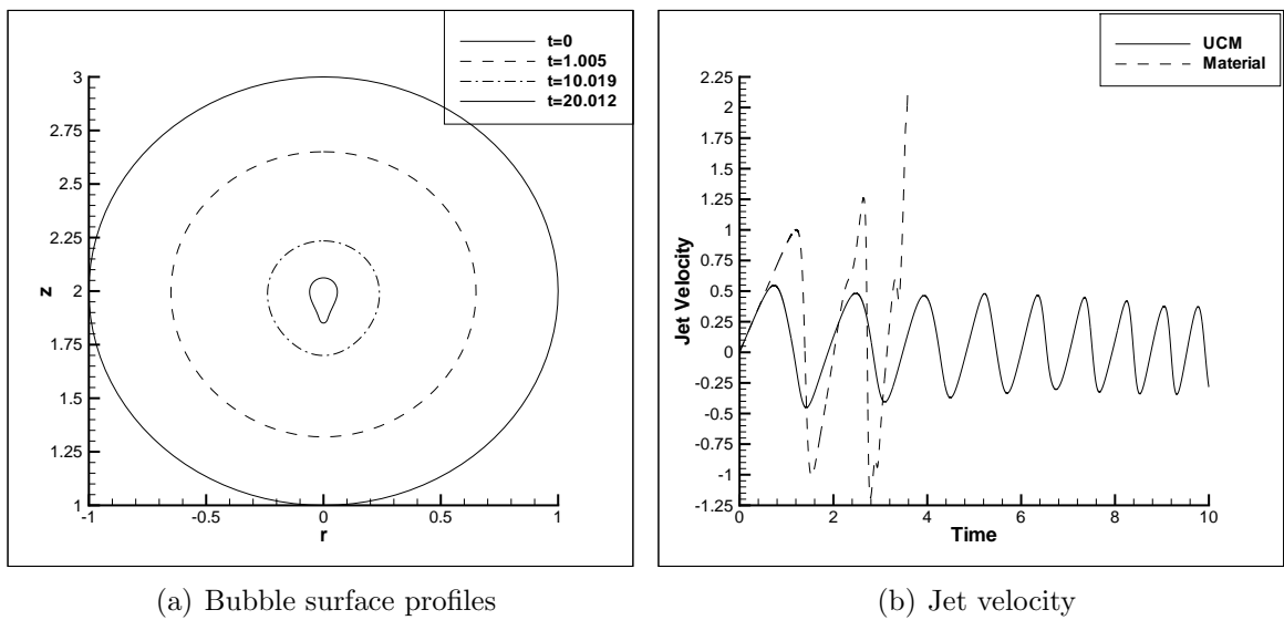
Figure 3.35: Bubble collapse near a wall using the UCM model. De = Re = 1 , h = 2
