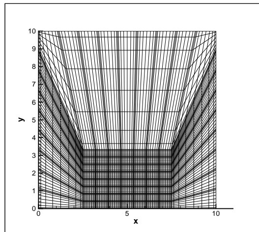
Figure 7.14: An example of the spectral element mesh used in the bubble collapse problems.
