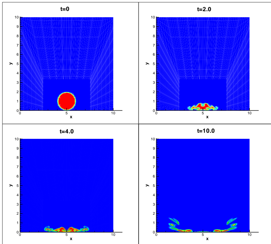
Figure 7.15: Bubble collapse near a wall in a Newtonian fluid with \mu_s = 1 \times 10^{-3} .
