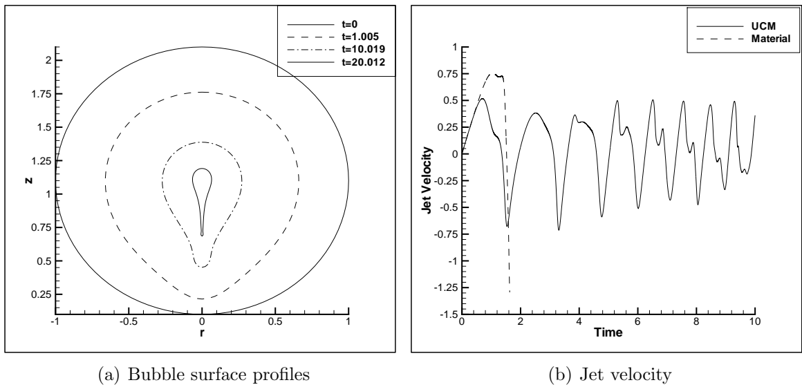
Figure 3.34: Bubble collapse near a wall using the UCM model. De = Re = 1 , h = 1.1
