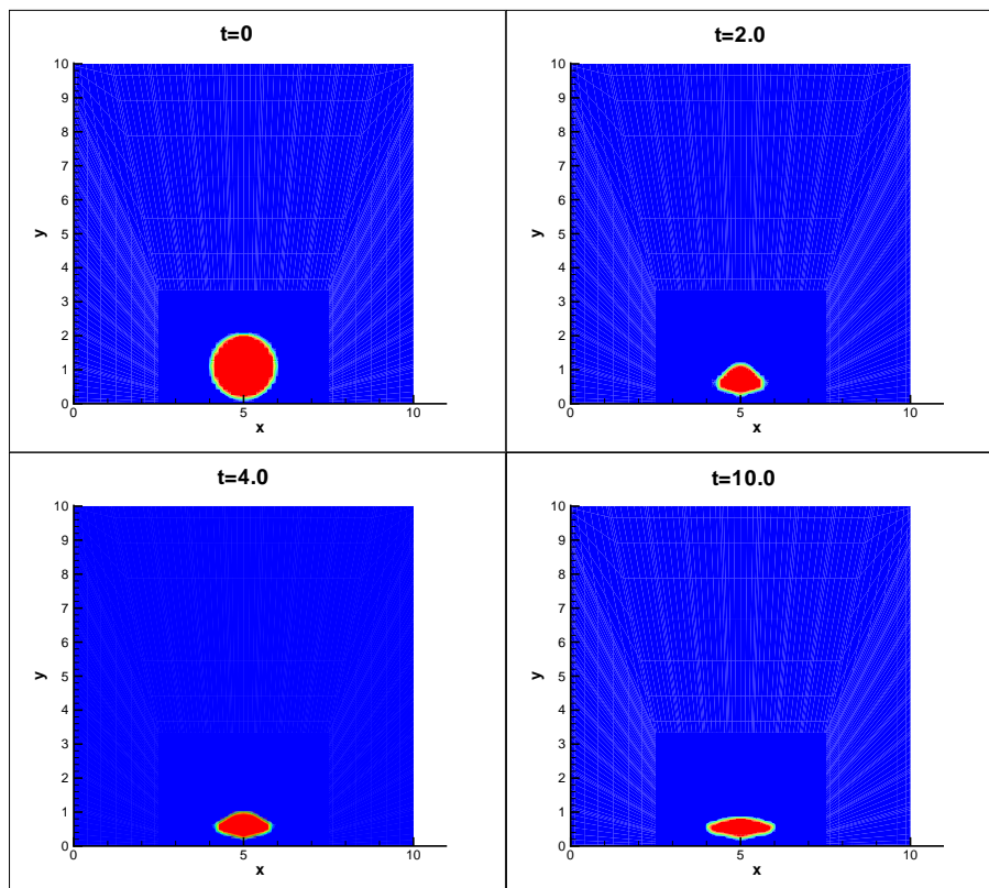
Figure 7.21: A plot of the colour function at different times, representing bubble collapse near a wall in a Newtonian fluid with \mu_s = 0.1 , h = 1.1 .
