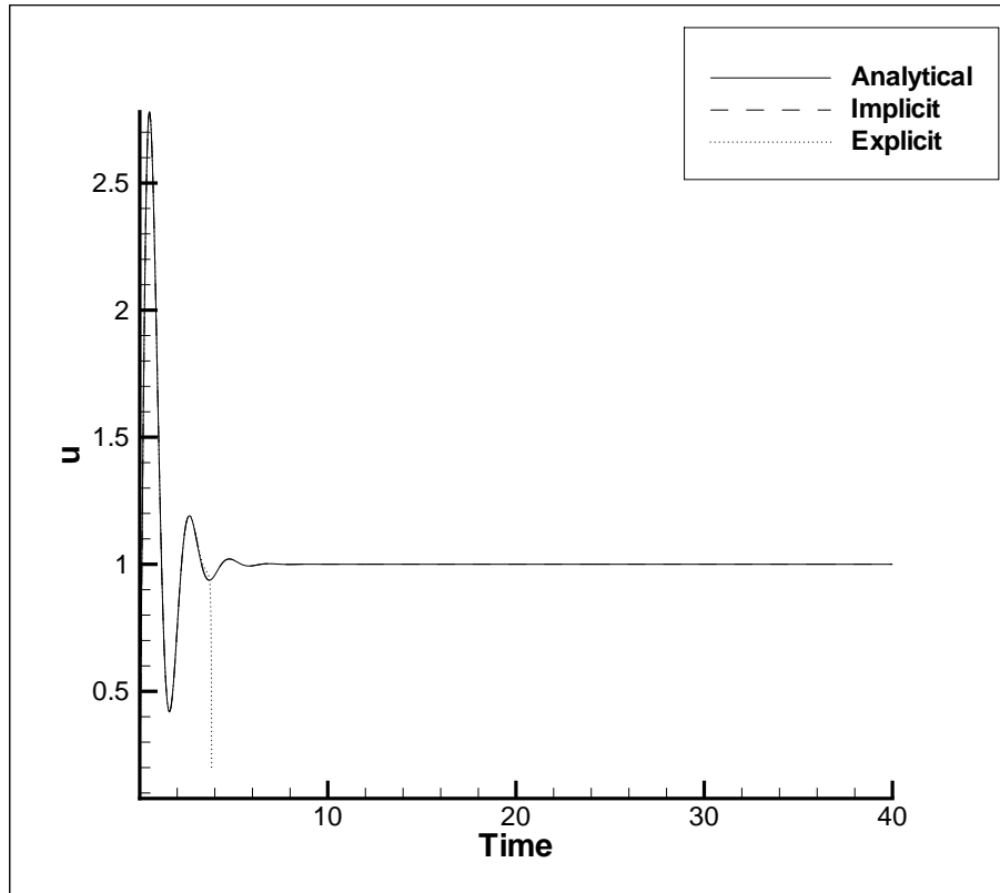
Figure 7.10: Analytical and numerical component of velocity u with time for an Oldroyd B fluid in Poiseuille flow. L = 8 , We = 1 , Re = 1 , \beta = 1/9 . The grid parameters are: N = 6 , \alpha = 1 , \beta = 1
