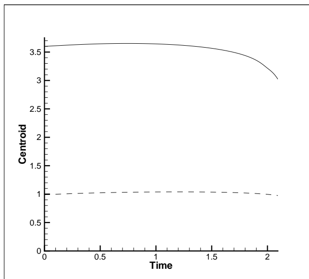
Figure 4.4: Evolution of bubble centroids. h_2 = 0.99 , h_1 = 3.60 , R_1 = 0.94
