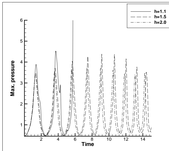
Figure 3.42: Variation of maximum pressure with time at different heights: Re = 0.2 , De = 5 .
