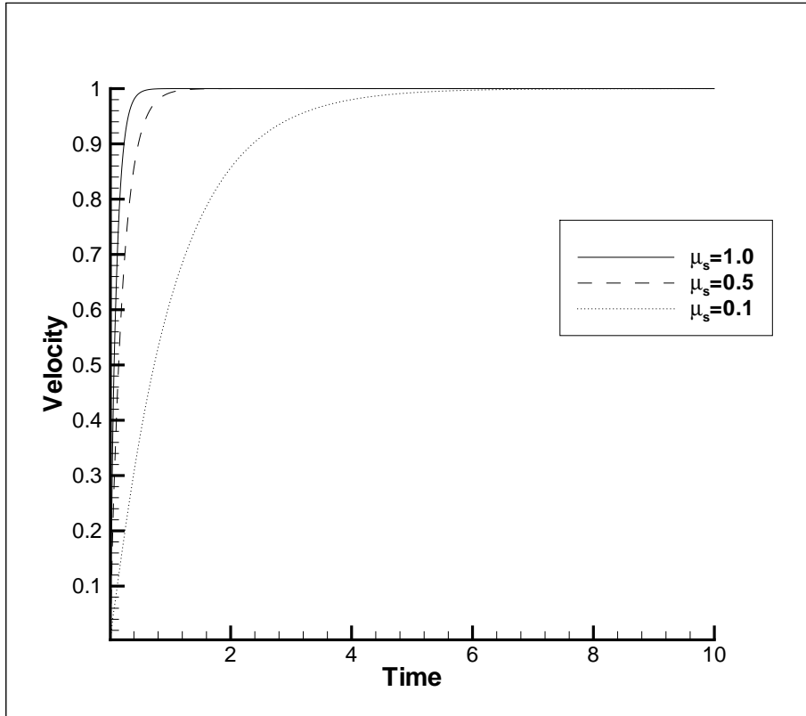
Figure 7.7: Numerical approximation of horizontal velocity component u(0.5, 0.5, t) with time for Poiseuille flow. Here c^2 = 1 \times 10^3 and the channel length is L = 1 .
