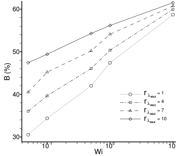
Figure 5.26: Dependence of the swelling ratios on Weissenberg number for different values of r_{\lambda_{max}} , with \lambda_1 = \lambda_2 = \lambda_3 = 10^{-3} , \lambda_4 = 10^{-1} .
