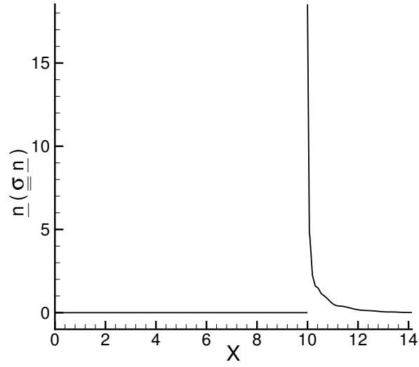
Figure 4.16: Axial normal stress profile on the free surface.
