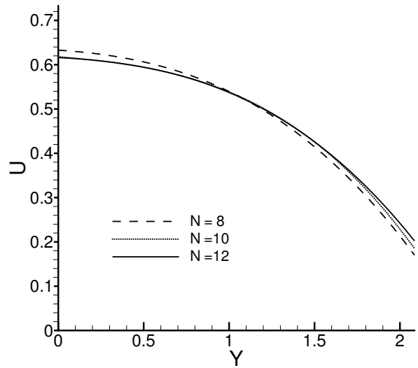
Figure 4.20: Horizontal velocity profiles at x = 8 (top) and x = 10.2 (bottom) with M = 4 , Re = 1 .
