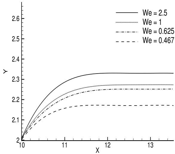
Figure 4.34: Free surface profiles for different values of surface tension for Re = 1 and N = 12 .
